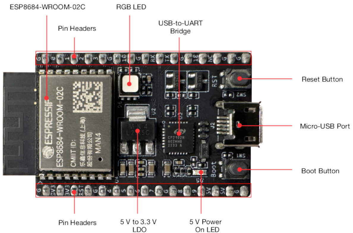
ESP8684-DevKitC-02 - front
