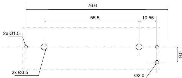
PCB MOUNTING LAYOUT
