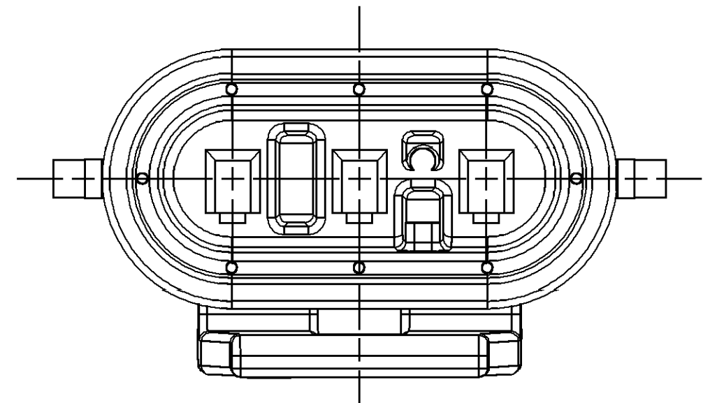
TYPE 104 SAME AS TYPE 101 EXCEPT AS SHOWN
