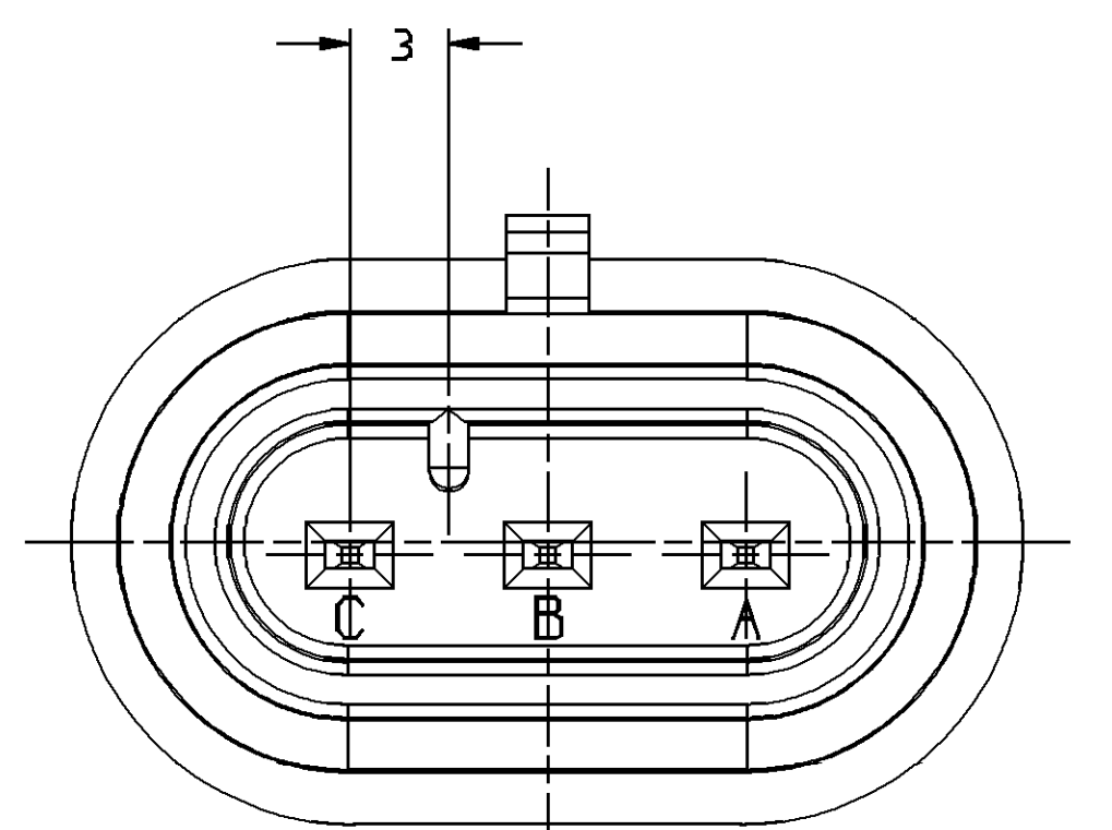
TYPE 102 SAME AS TYPE 101 EXCEPT AS SHOWN
