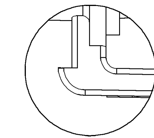
DETAIL Y SCALE 6:1 TYPE 102 & 103 SAME AS TYPE 101 EXCEPT AS SHOWN 2X-TYP
