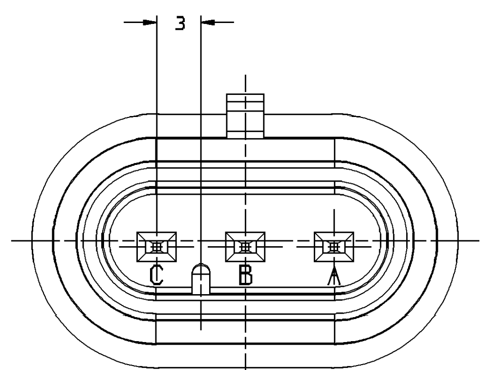
TYPE 103 SAME AS TYPE 101 EXCEPT AS SHOWN
