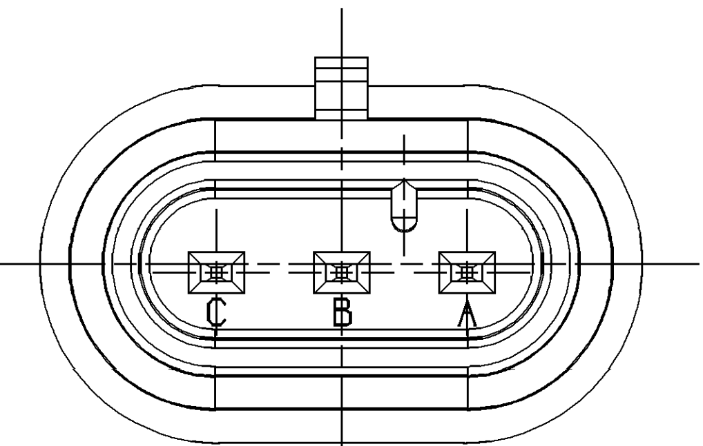
TYPE 104 SAME AS TYPE 101 EXCEPT AS SHOWN
