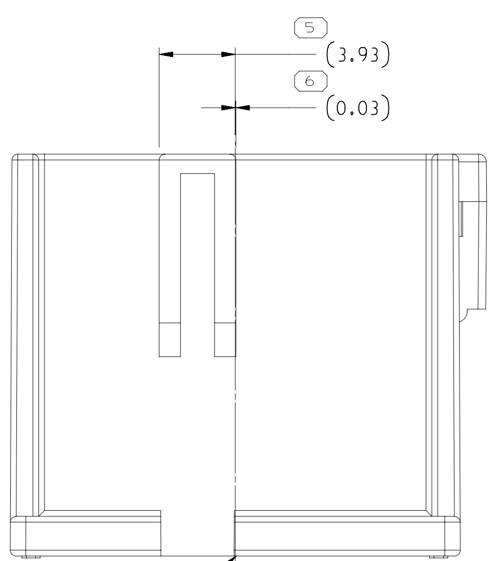
TYPE 106 SAME AS TYPE 101 EXCEPT AS SHOWN
