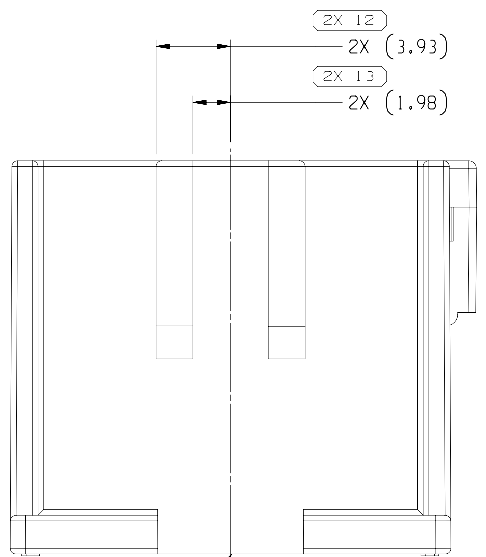
TYPE 105 SAME AS TYPE 101 EXCEPT AS SHOWN
