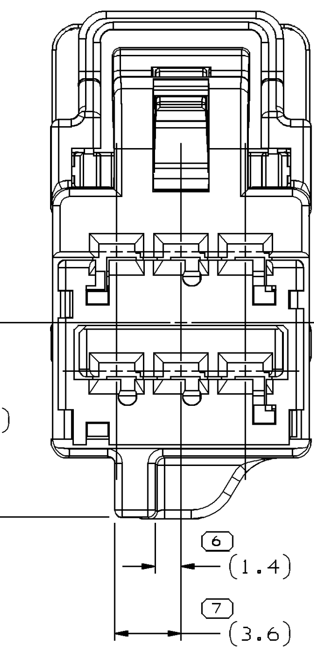
TYPE 104 SAME AS TYPE 101 EXCEPT AS SHOWN
