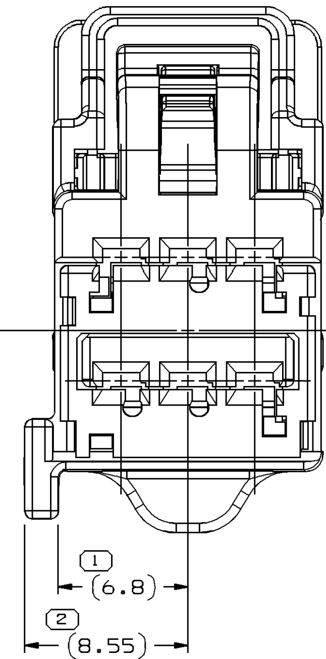
TYPE 102 SAME AS TYPE 101 EXCEPT AS SHOWN
