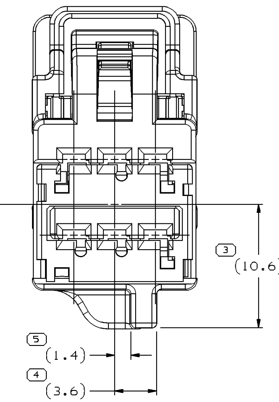
TYPE 103 SAME AS TYPE 101 EXCEPT AS SHOWN
