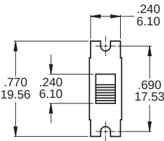
"B" WITH MOUNTING EARS
