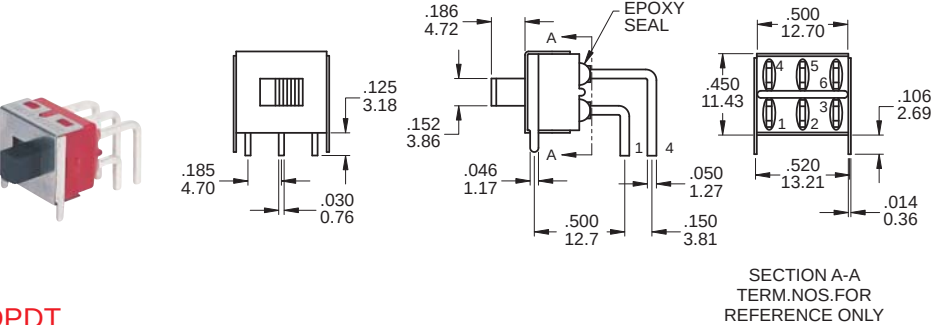
DPDT
