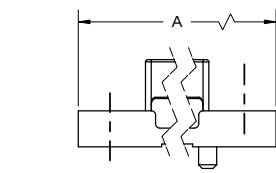
MOUNTING CODE: 02
