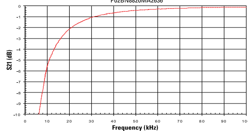
Opti-Cap Low Frequency Insertion Loss, (S21) P02BN820MA2636
