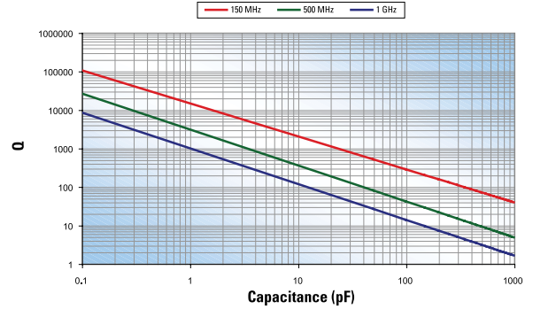
Q vs Capacitance DLI C18 AH Series
