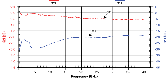
Opti-Cap Insertion & Return Loss, (S21 & S11) P02BN820MA2636
