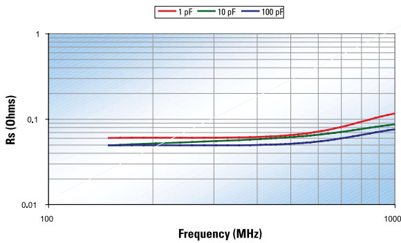
ESR vs Frequency DLI C17 AH Series
