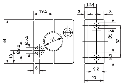
Flange for M18
