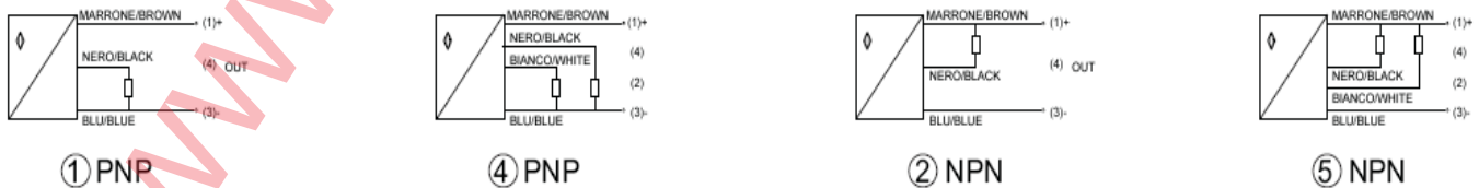
Wiring Diagram
