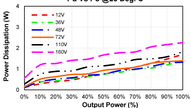
EC7AW18-72D05 Pd Vs Po @25 Deg. C
