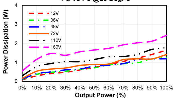
EC7AW18-72S15 Pd Vs Po @25 Deg. C
