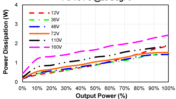
EC7AW18-72D12 Pd Vs Po @25 Deg. C
