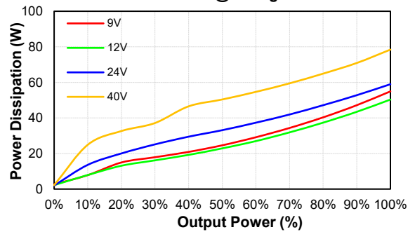
CHB500W-24S54 Pd Vs Po @25 Deg. C
