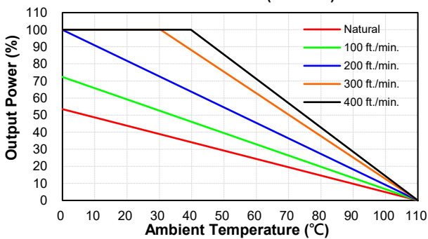
CHB500W-24SXX Derating Curve with Heatsink HBT127 (Vin=24V)
