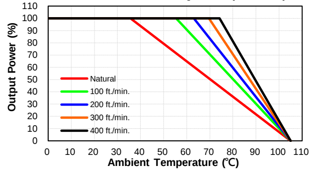
CQB100W14-72S15, 24, 28, 54 Derating Curve with Heatsink QBL127 (Vin=72V)
