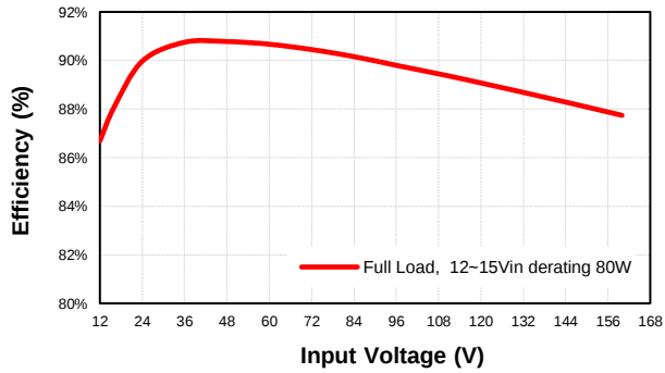
CQB100W14-72S28 Eff Vs Vin @25 Deg. C
