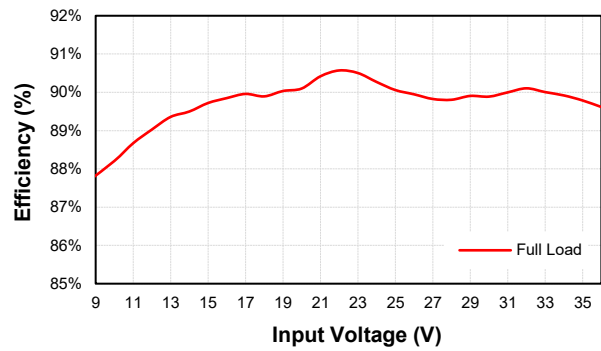
CQM60W-24D15 Eff Vs V_{in} @25 Deg. C
