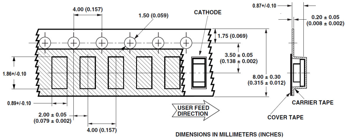
Figure 10: Carrier Tape Dimensions
