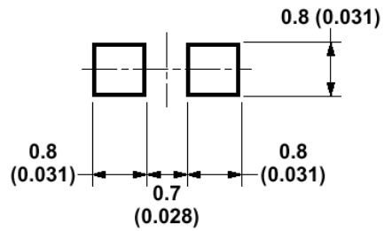
Figure 9: Recommended Soldering Land Pattern
