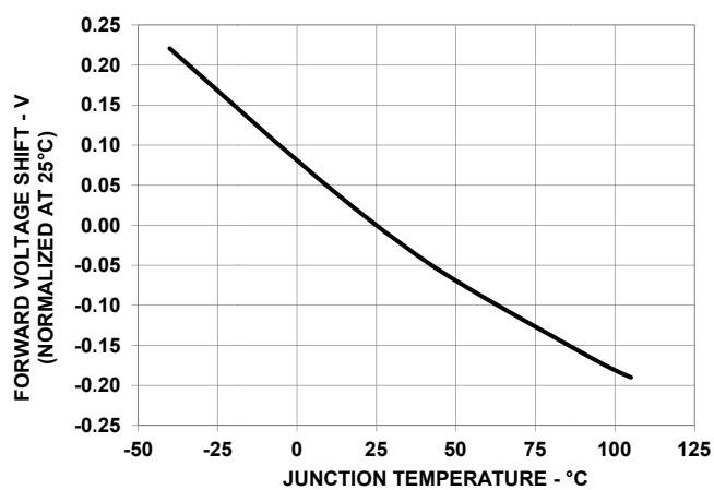
Figure 4: Forward Voltage vs. Temperature
