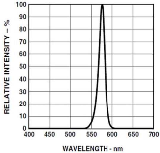
Figure 2: Spectral Power Distribution
