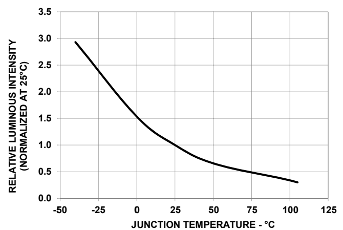
Figure 5: Luminous Intensity vs. Temperature
