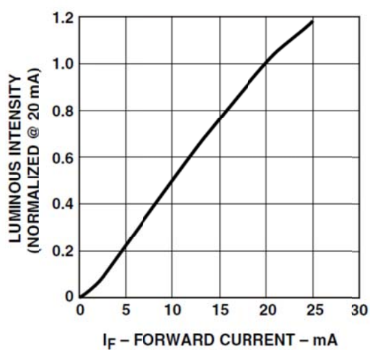
Figure 6: Relative Luminous Intensity vs. Forward Current
