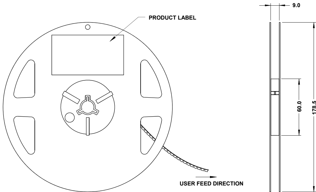
Figure 11: Reel Dimensions
