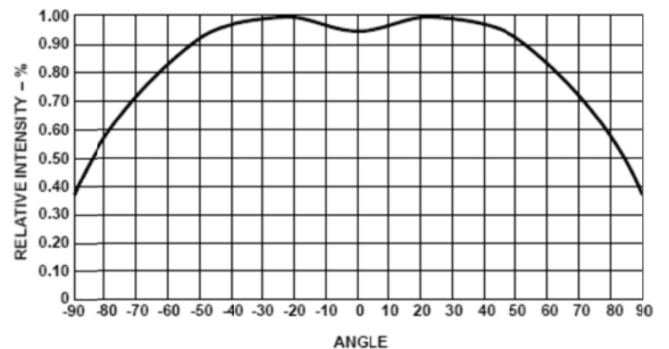
Figure 7: Radiation Pattern
