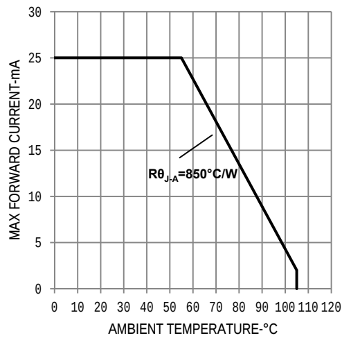
Figure8: Derating Curve
