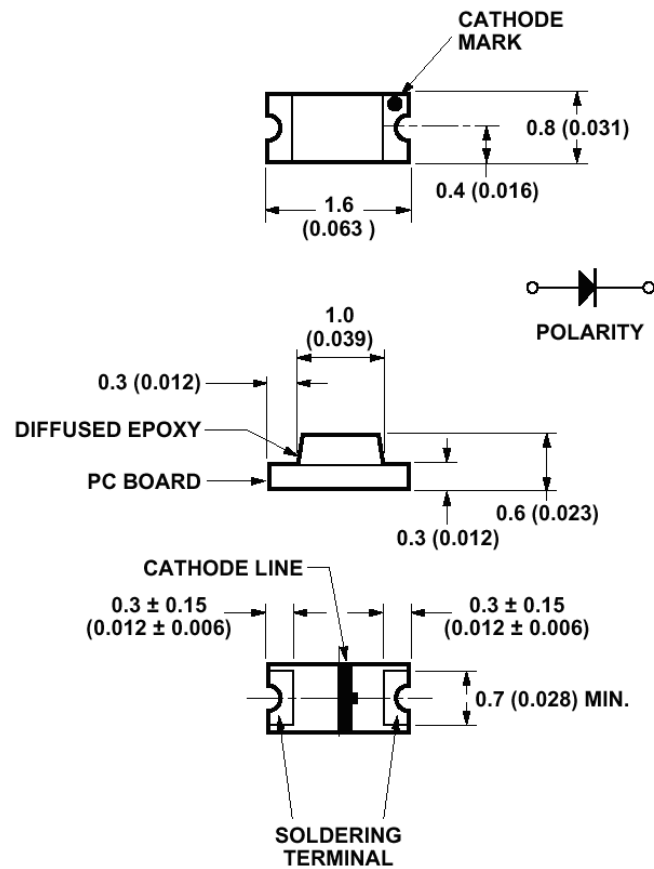
Figure 1: Package Dimensions
