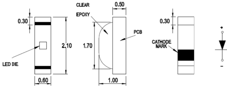
Figure 1: Package Dimensions
