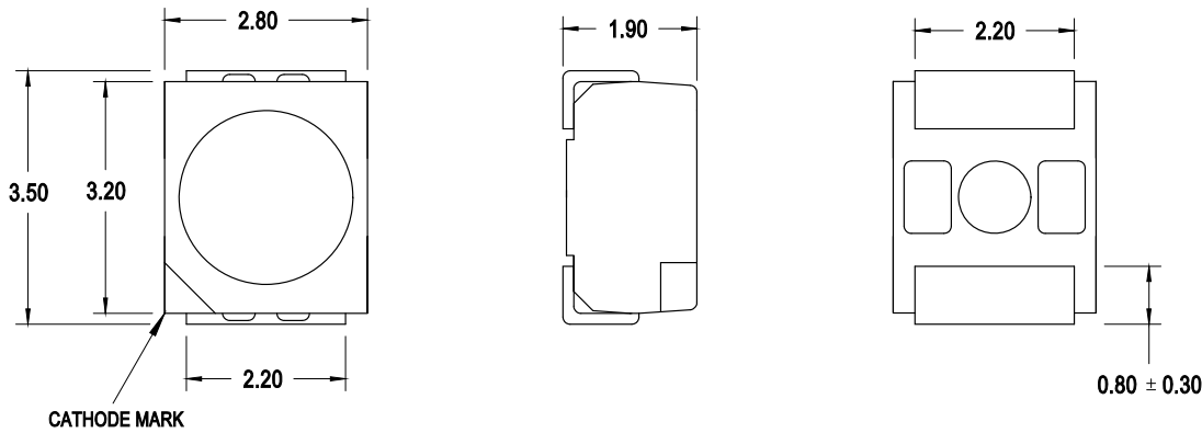
Figure 1: Package Drawing
