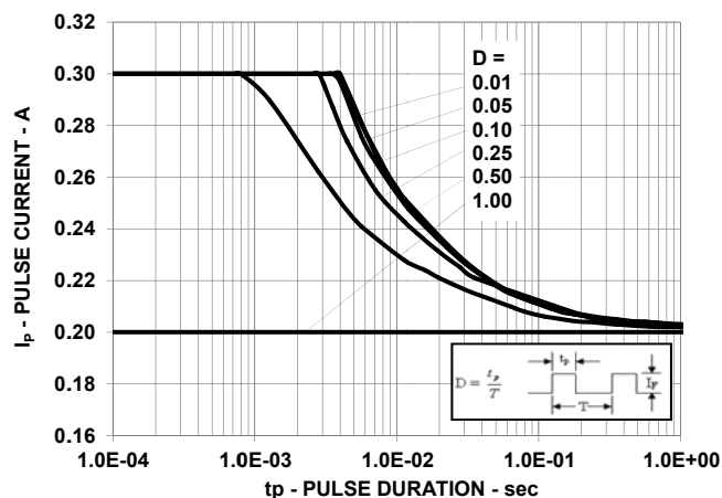
Figure 14: Pulse Handling Capability at T_s \leq 100^{\circ}\text{C} (Far Red)
