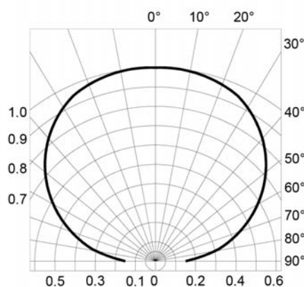
Fig. 4 Directivity Radiation Diagram
