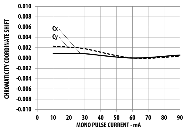
Figure 6: Chromaticity Coordinate Shift vs. Mono Pulse Current for 4000K.
