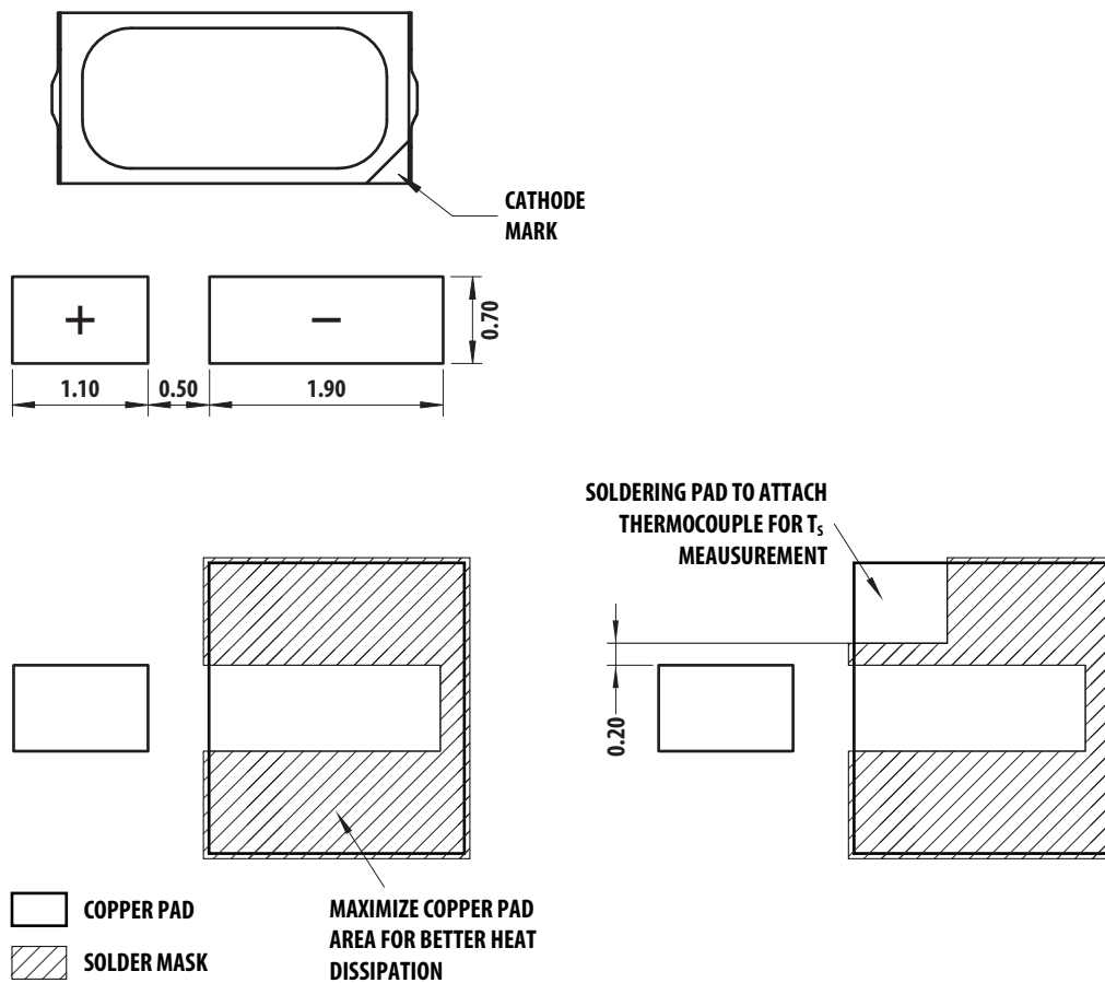
Figure 15: Recommended soldering pad pattern.
