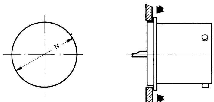
Mounting hole
