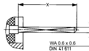
Detail X
