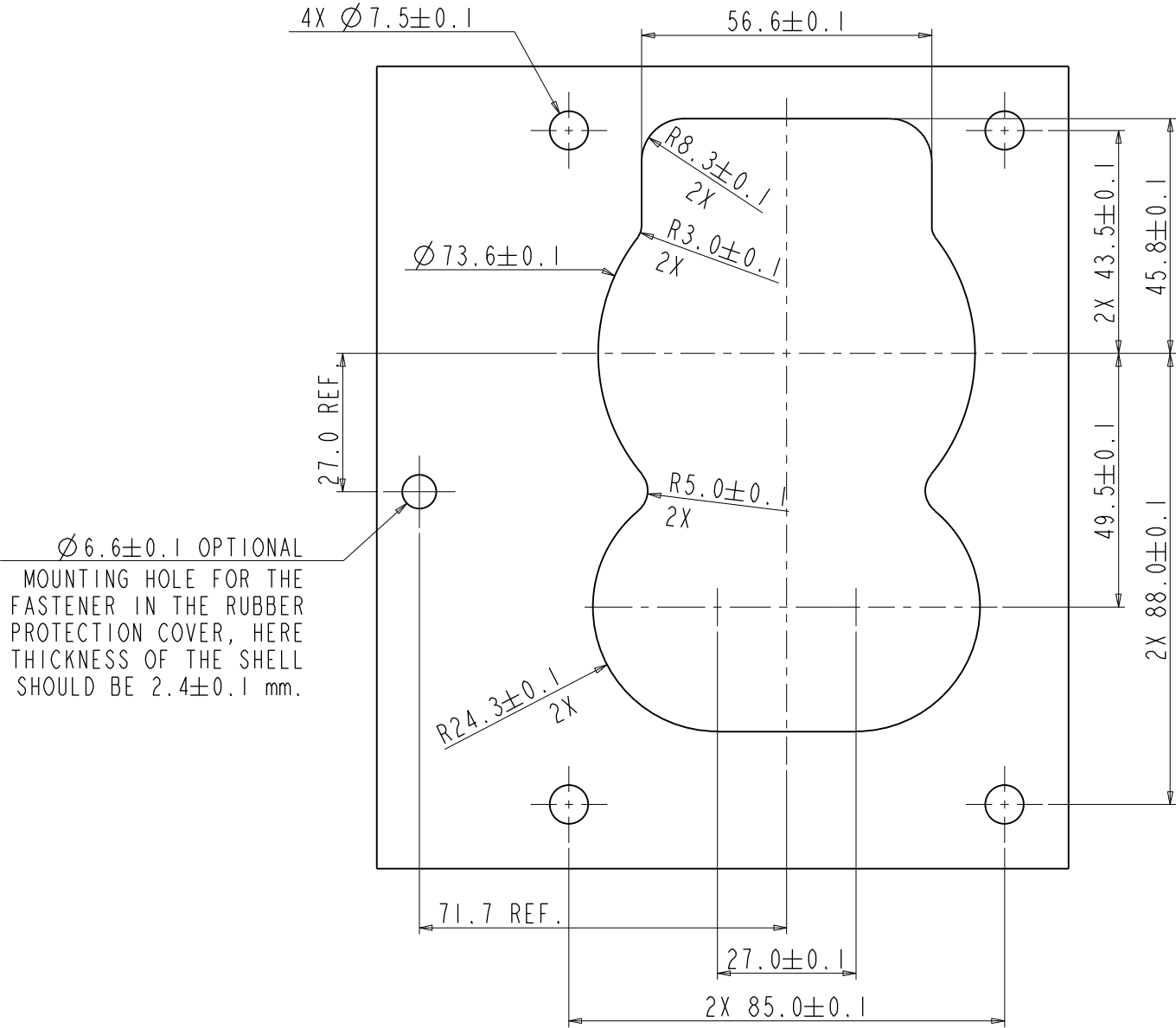
FIGURE 1 RECOMMENDED HOLE LAYOUT IN MOUNTING PANEL RECOMMENDED MIN. WALL THICKNESS: 3.0±0.1 mm
