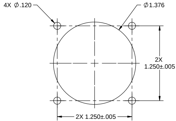
PANEL CUT-OUT DIMENSIONS
