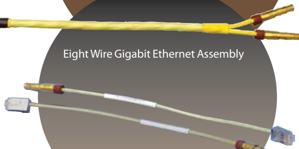
Quadrx Contact with 8P8C "RJ45" Jack Ethernet Assembly
