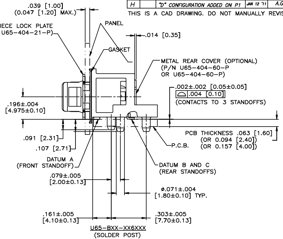
DIMENSION TABLE:
