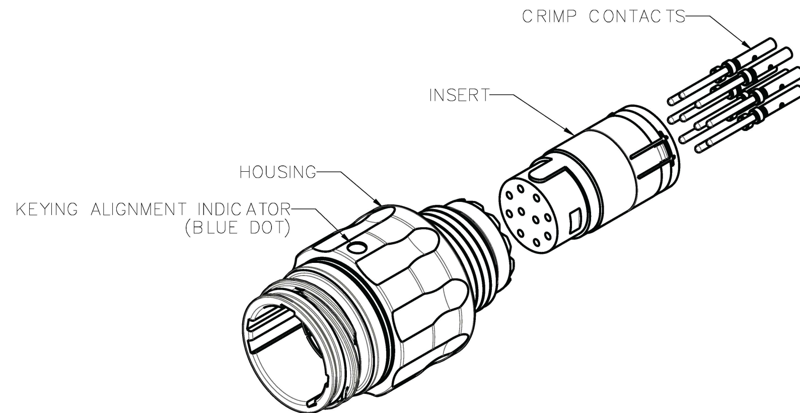
ISOMETRIC VIEW FOR REFERENCE ONLY TMR-LTAN09-010APC00A SHOWN
