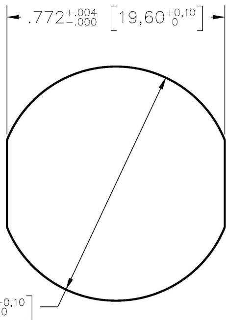
PANEL CUTOUT
