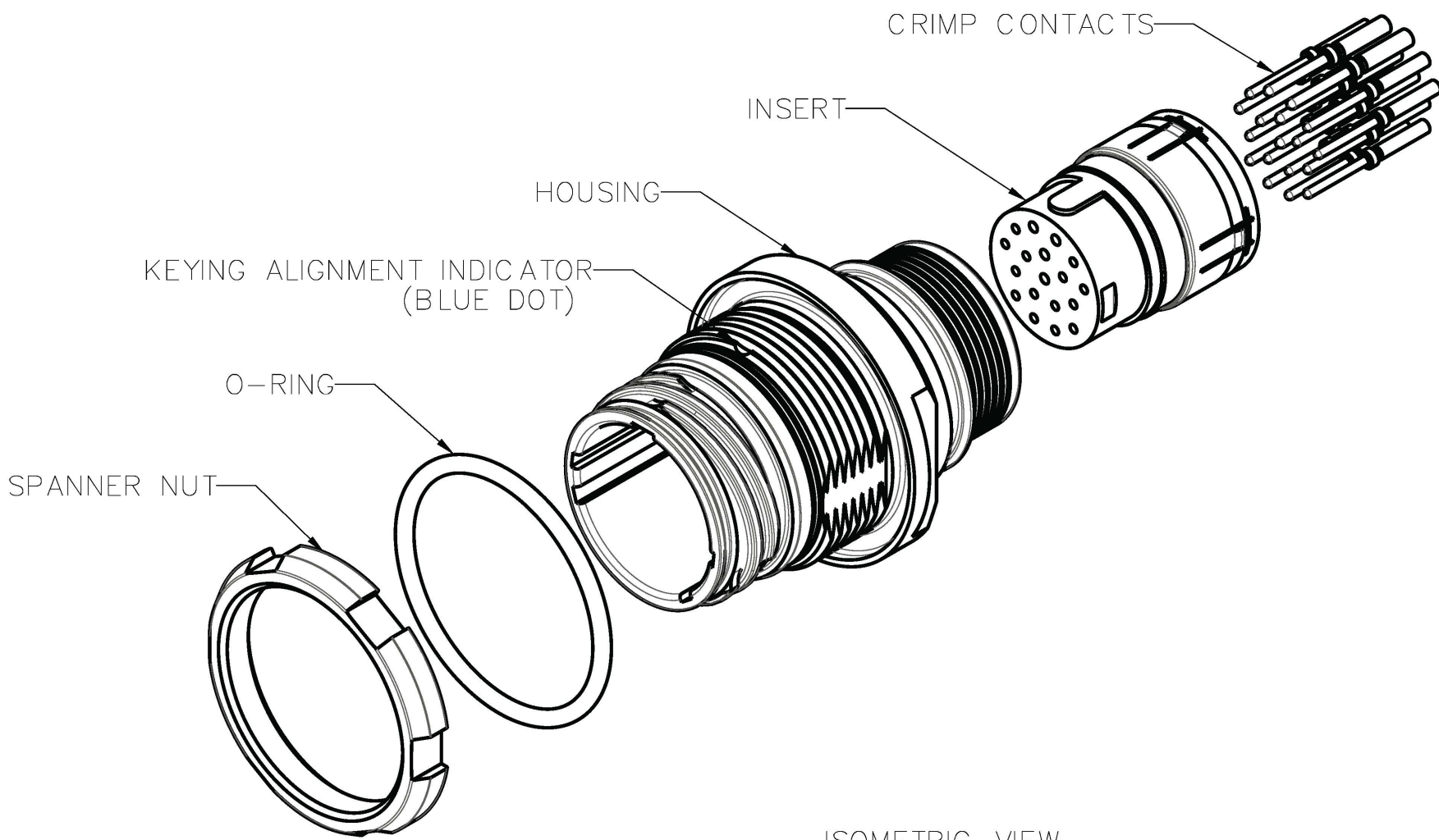
ISOMETRIC VIEW FOR REFERENCE ONLY TMR-JSAN12-018APC00A SHOWN
