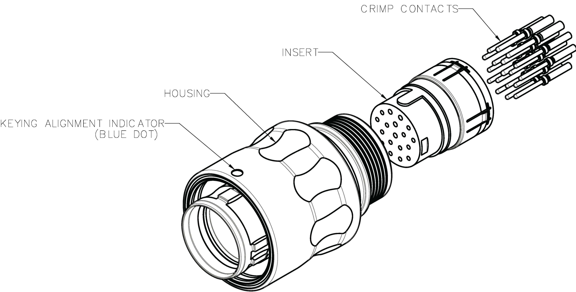
ISOMETRIC VIEW FOR REFERENCE ONLY TMP-B SAN12-018APC00A SHOWN
