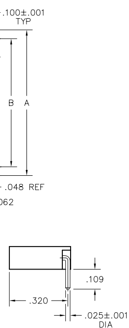
RIGHT ANGLE (WT8SAR7)
