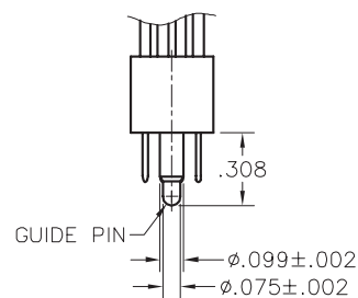
HARDWARE STYLE 57
