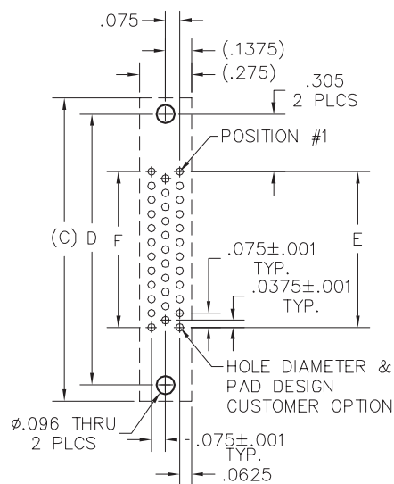
PCB LAYOUT VIEWED FROM COMPONENT SIDE
