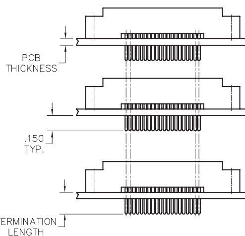
STACKED CONNECTORS
