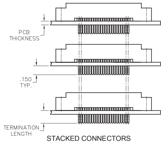
STACKED CONNECTORS
