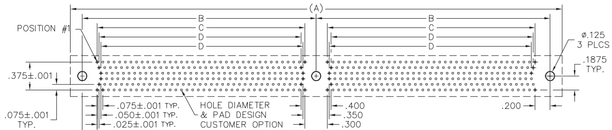
PCB LAYOUT VIEWED FROM COMPONENT SIDE
