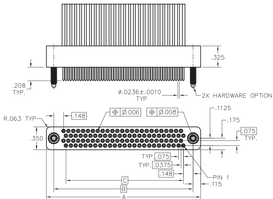
PLUG
