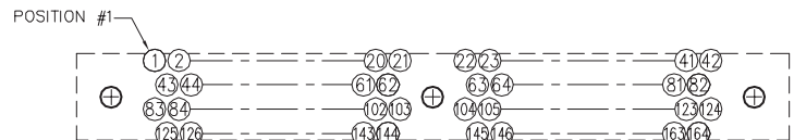
CONNECTOR PIN IDENTIFICATION PATTERN VIEWED FROM MATING FACE (EXAMPLE: 164 POSITION CONNECTOR)
