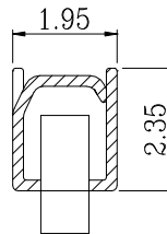
SEC C-C
