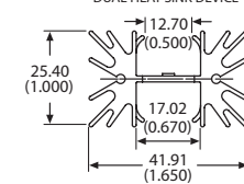
VIEW A-A DUAL HEAT SINK DEVICE
