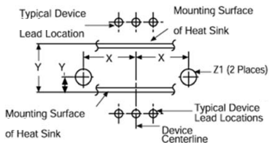
Mounting Details:
