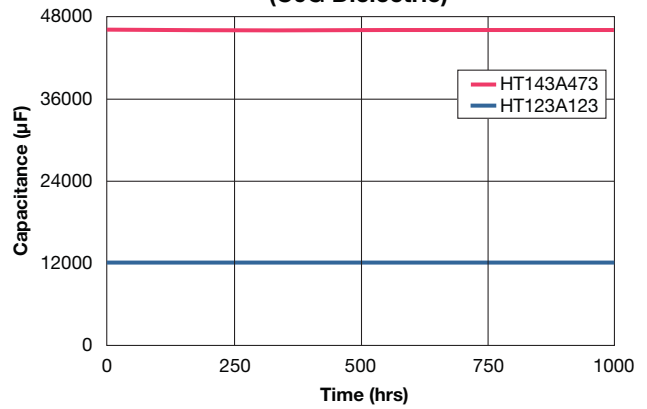
250°C Life Test @ 2x Rated Voltage (COG Dielectric)
