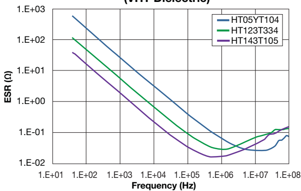
ESR Frequency Response (VHT Dielectric)
