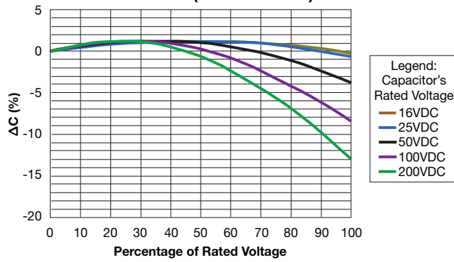
Typical Voltage Coefficient of Capacitance (VHT Dielectric)
