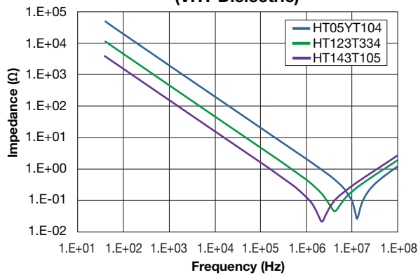
Impedance Frequency Response (VHT Dielectric)
