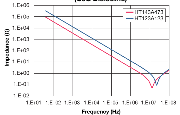
Impedance Frequency Response (COG Dielectric)
