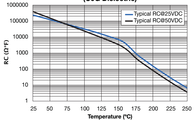
RC vs Temperature (C0G Dielectric)
