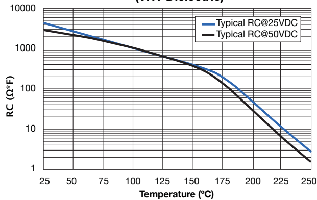
RC vs Temperature (VHT Dielectric)
