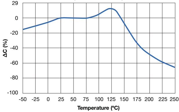
Typical Temperature Coefficient of Capacitance (VHT Dielectric)
