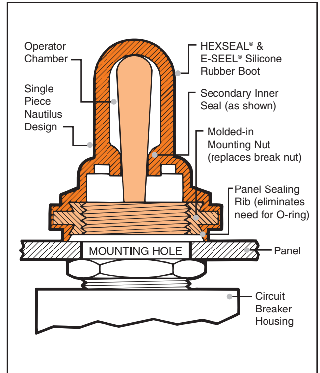
Full-Toggle Boot with Integral Secondary Inner Seal – IP66/68 Rated
