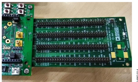
Figure 15. EI3 SDP Breakout Board Connected to EZ-Kit Board
