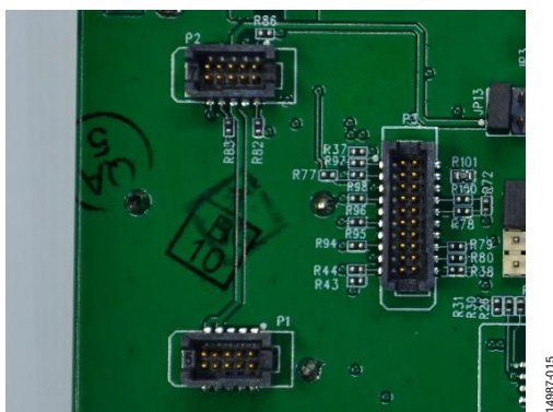
Figure 16. Wireless Transceiver Interface
