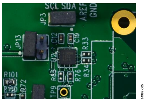
Figure 6. Tri Sensor Circuit
