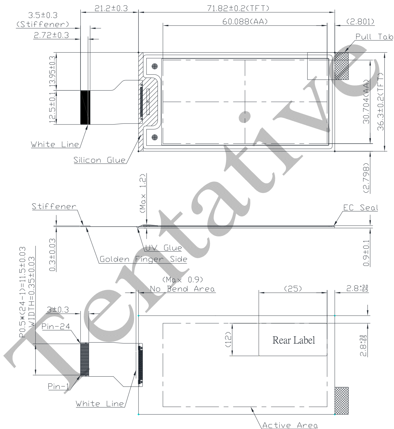
Figure 1-1 EPD Drawing
