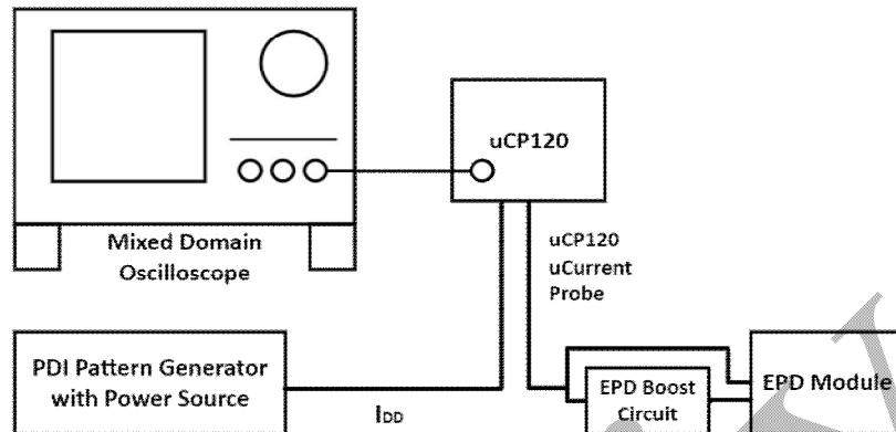
Figure 3-3 Current Measurement
