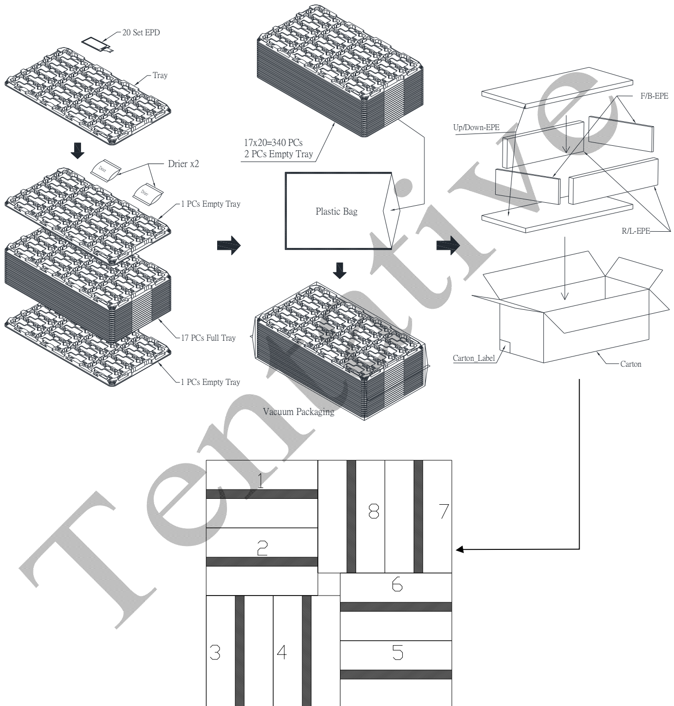
Figure 7-1 Packing Diagram
