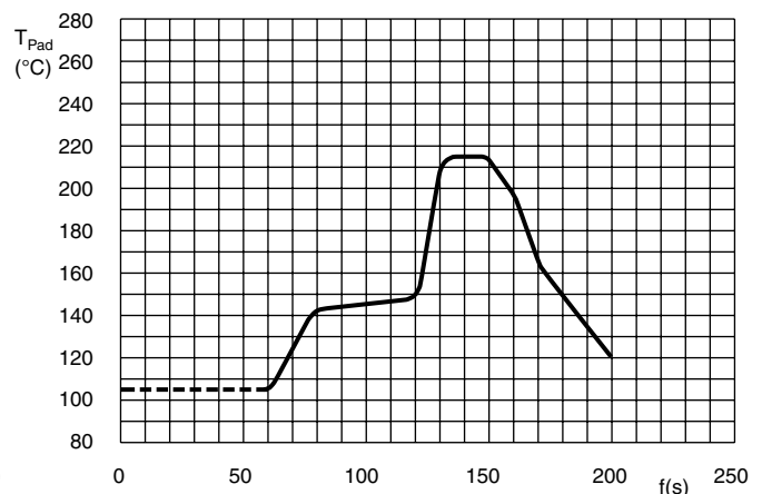
Fig.6 Maximum temperature load during vapor phase reflow soldering
