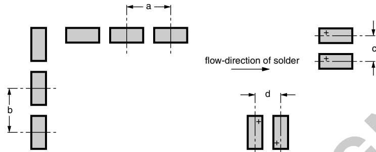
Fig.4 Minimum distances between 085 CS capacitors on a printed-circuit board for wave soldering
