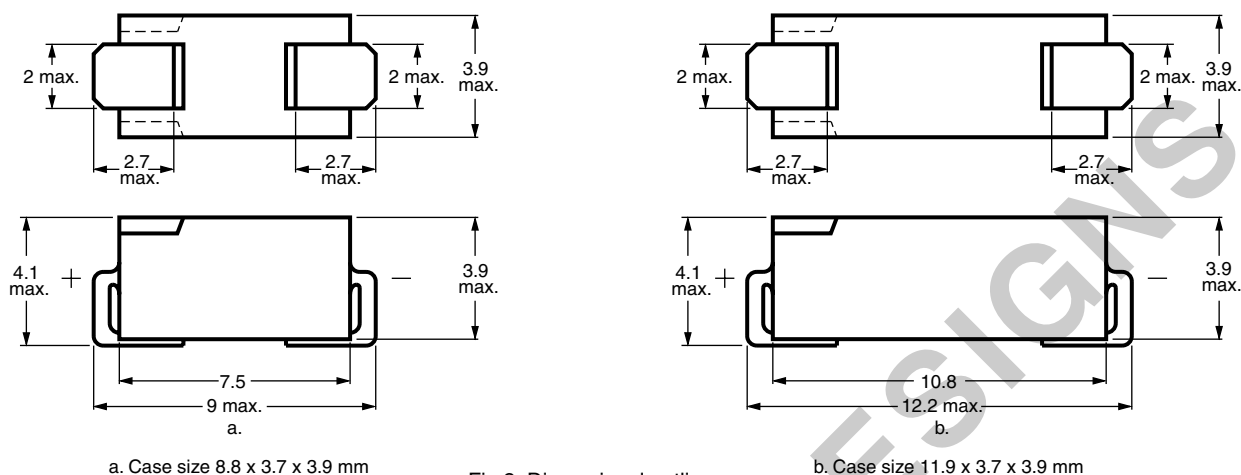
Fig.2 Dimensional outlines
