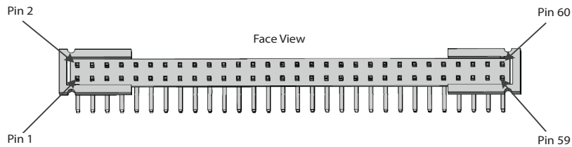
Figure 1-4: Video Header
