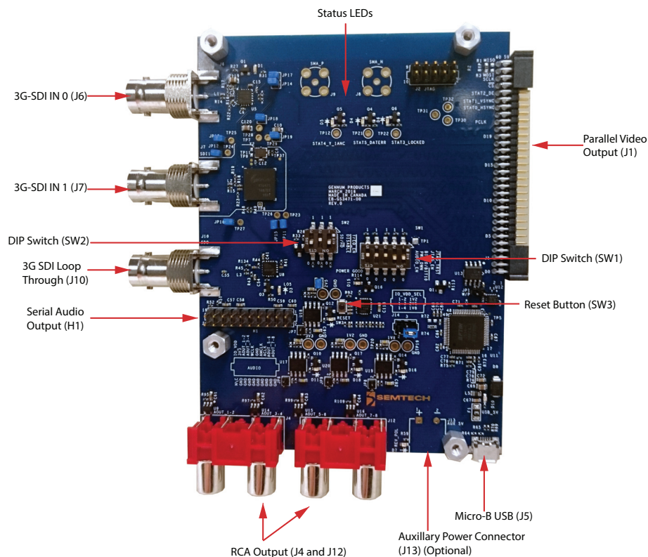
Figure 1-1: GS3471 Evaluation Board (EB-GS3471-00)
