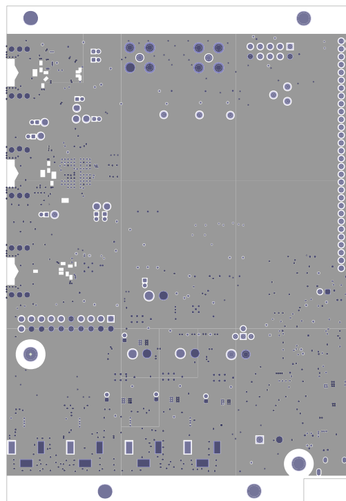
Figure 3-4: Layer 4 (GND2)
