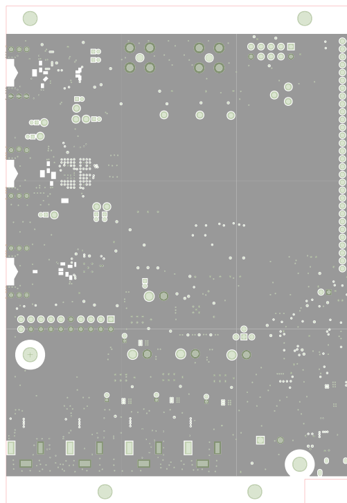
Figure 3-2: Layer 2 (GND1)
