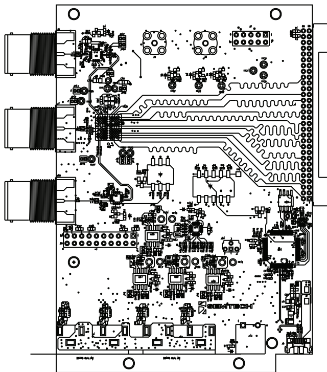
Figure 3-1: Layer 1 (TOP)
