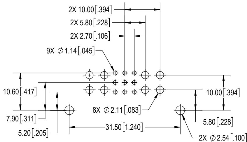
CONTACT HOLE PATTERN
