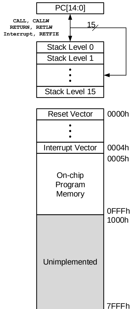
Figure 9-1. Program Memory and Stack (PIC16F152x4)
