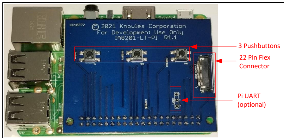
Figure 4: IA8201 Raspberry Pi Adapter Board connected to the Pi
