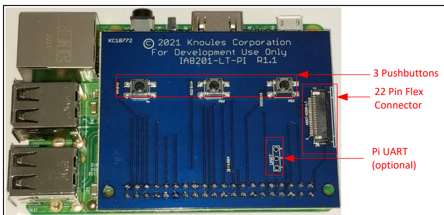
Figure 8: IA8201 Raspberry Pi Adapter Board connected to the Pi.
