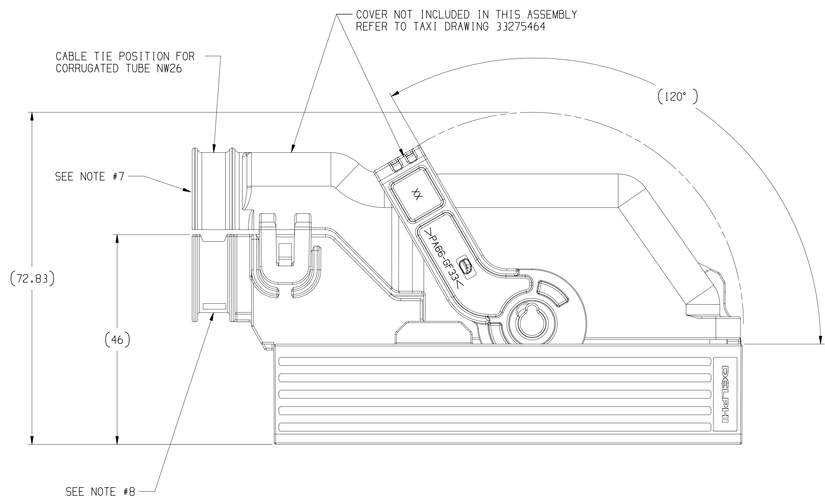
TYPE 104 SAME AS TYPE 10 EXCEPT AS SHOWN
