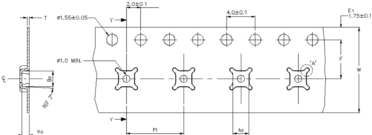
SECTION Y-Y
