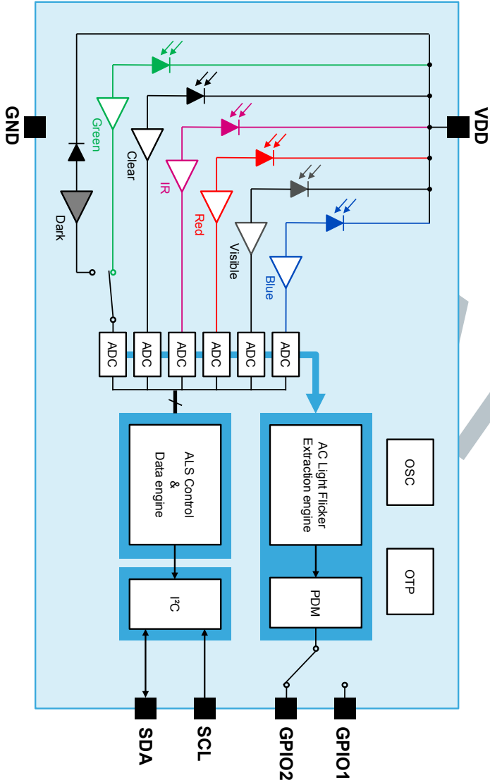
Figure 1. System block diagram (full options)
