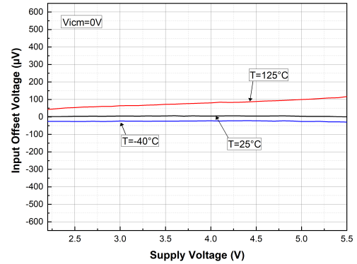
Figure 11. Input offset voltage vs. supply voltage
