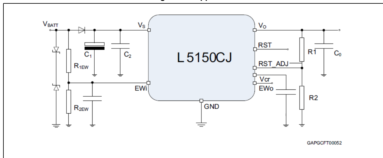
Figure 21. Application schematic
