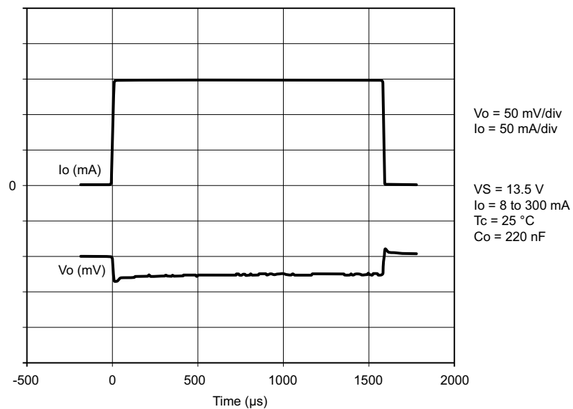
Figure 23. Maximum load variation response
