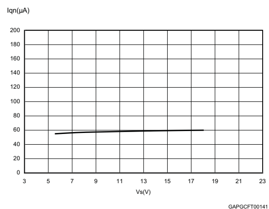
Figure 8. Current consumption vs. input voltage ( I_o = 0.1\text{mA} )
