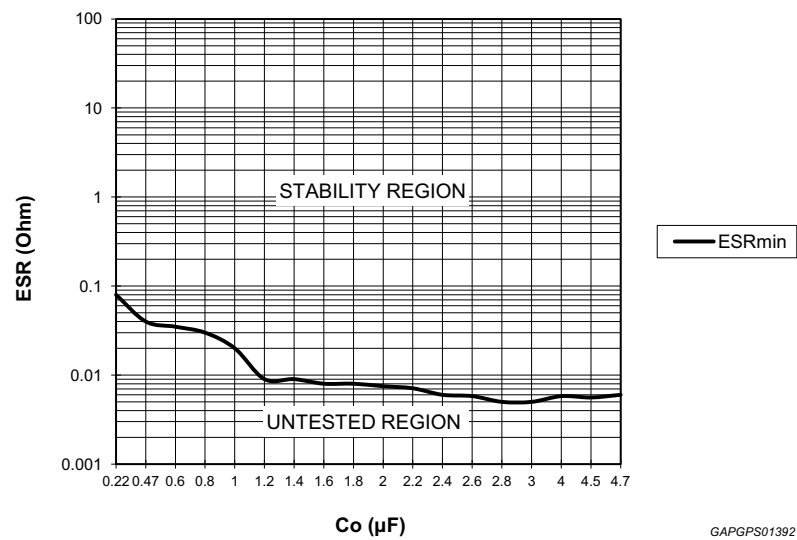
Figure 22. Stability region
