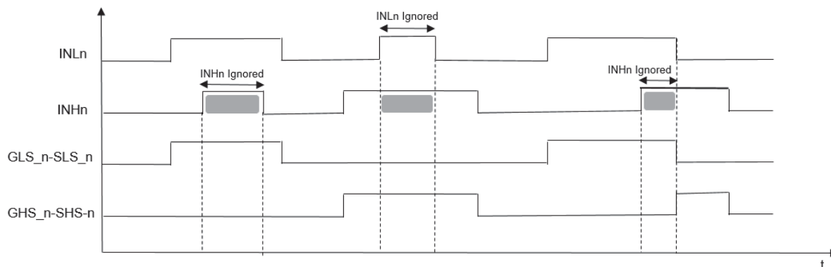
Figure 41. Interlocking protection on PWM inputs: functional operation
