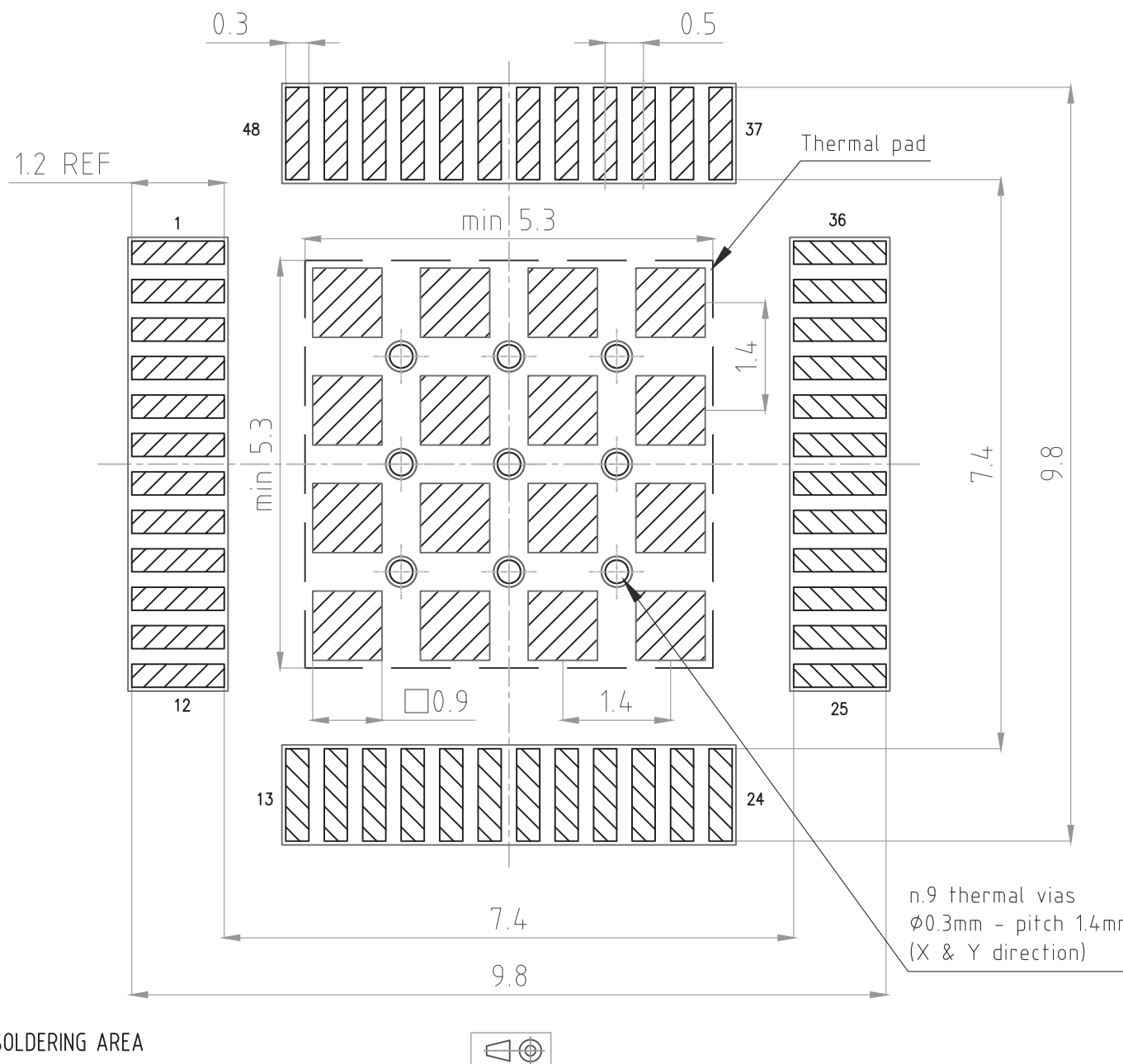
Figure 93. Suggested PCB landpattern
