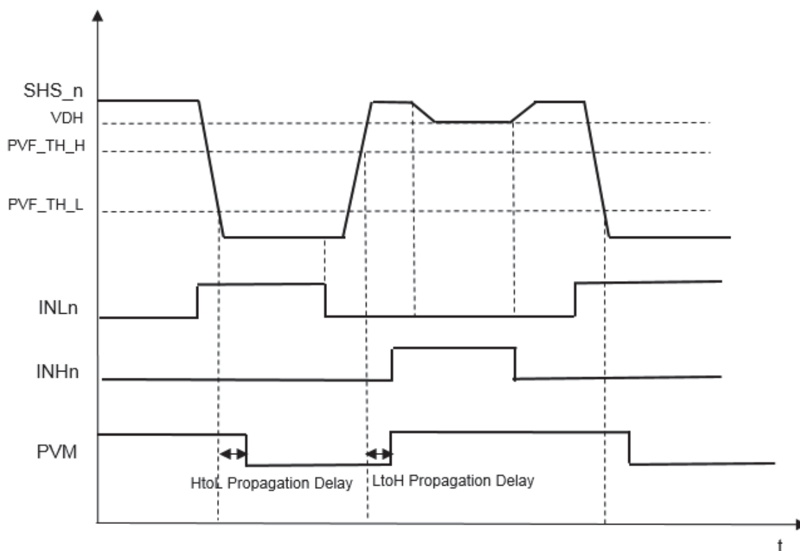
Figure 74. Phase voltage feedback behavior
