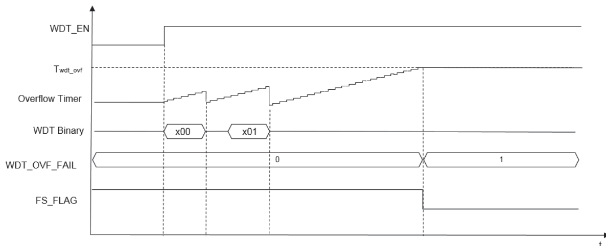
Figure 86. WDT Operation – Overflow timer failure
