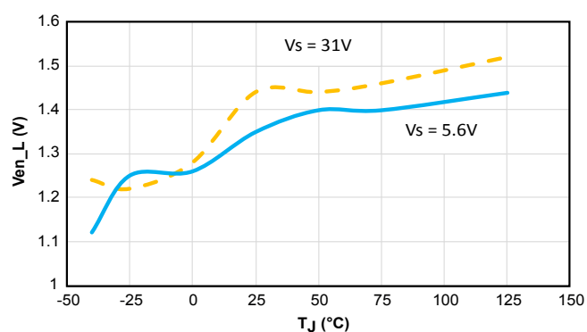
Figure 17. V_{En\_low} vs T_J
