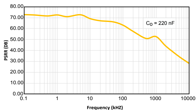
Figure 18. PSRR
