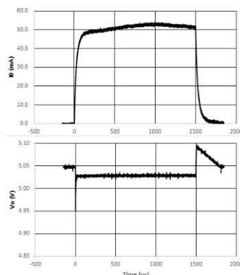
Figure 23. Maximum load variation response
