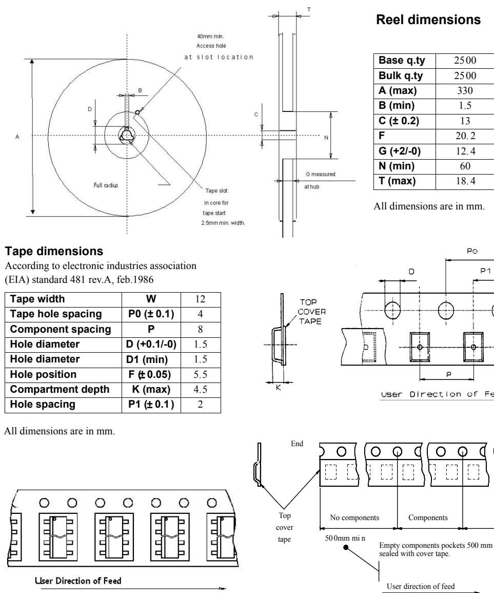
Figure 33. SO-8 tape and reel shipment (suffix "TR")
