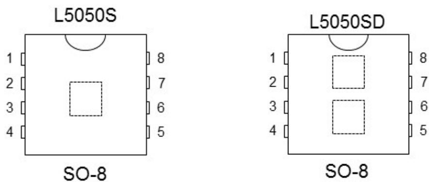
Figure 3. Pins configuration
