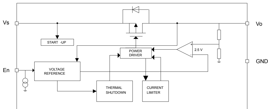
Figure 1. Functional block diagram - L5050S
